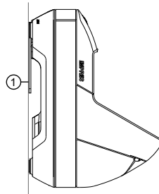
Figure 23: Charger Mounted on Wall Bracket
